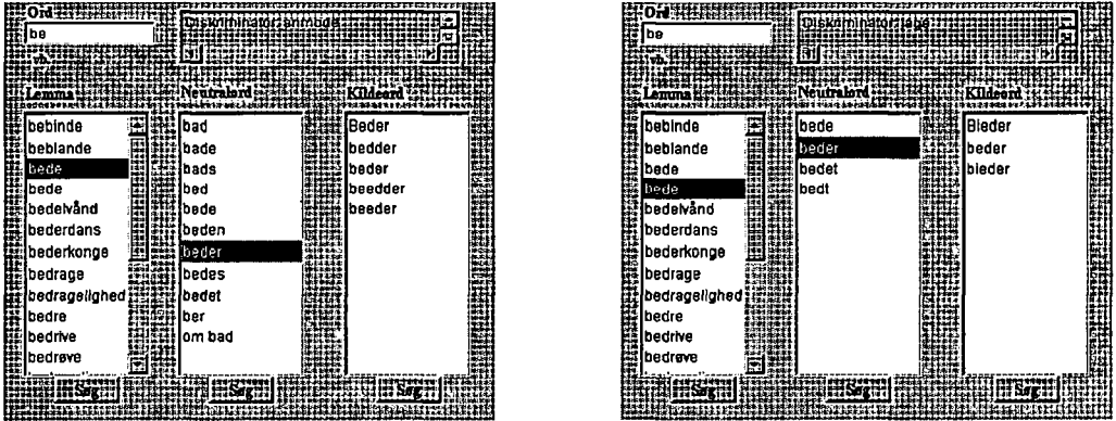
Figure 4: Look-ups of the two verbs bede ; the lemmalist is in the column to the left, the orthographically neutral forms of the selected lemma appear in the column in the middle, and the source forms of the selected neutral form in the column to the right.
